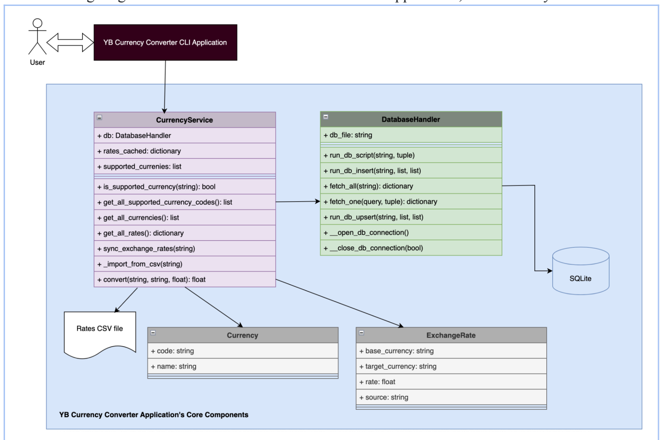
Figure 1. Overall architecture of YB Currency Converter
